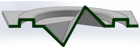
Figure 1: Section through the apices of the double tetrahedron moulding configuration with rotation.
